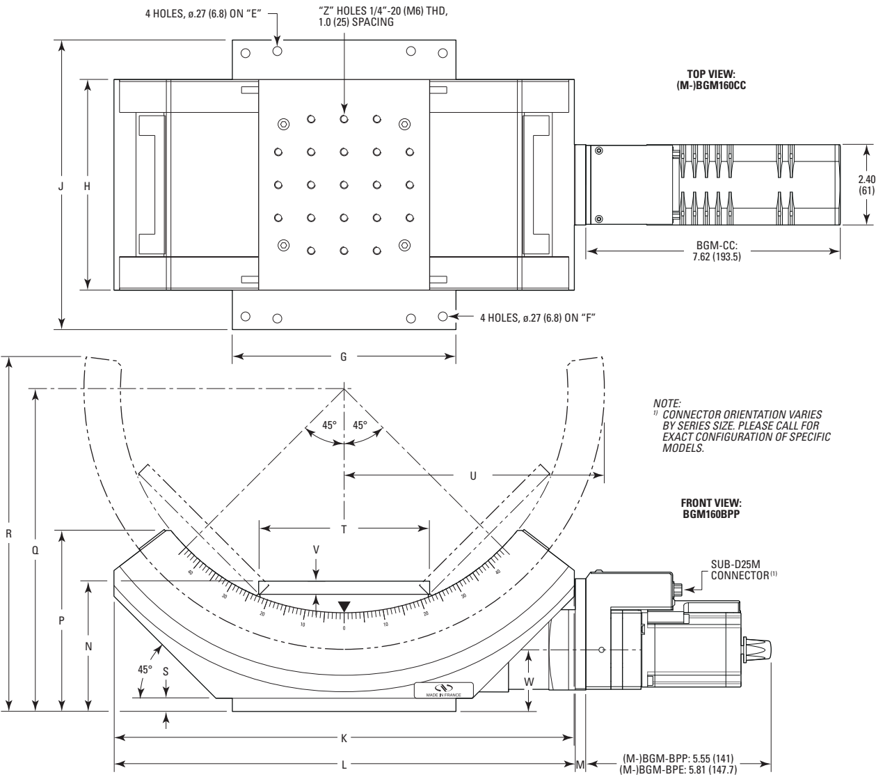
MODEL SHOWN: BGM160 DIMENSIONS IN INCHES (AND MILLIMETERS)
