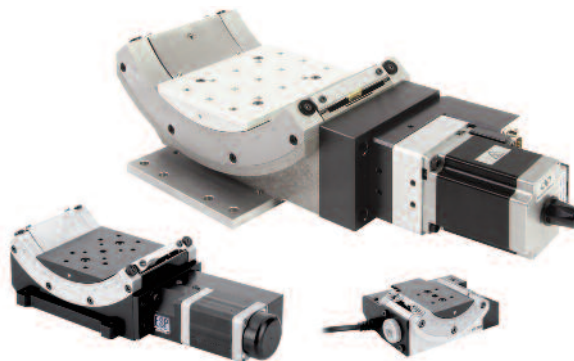
BGS50CC, BGS80PP and BGM120BPP goniometric cradles.
